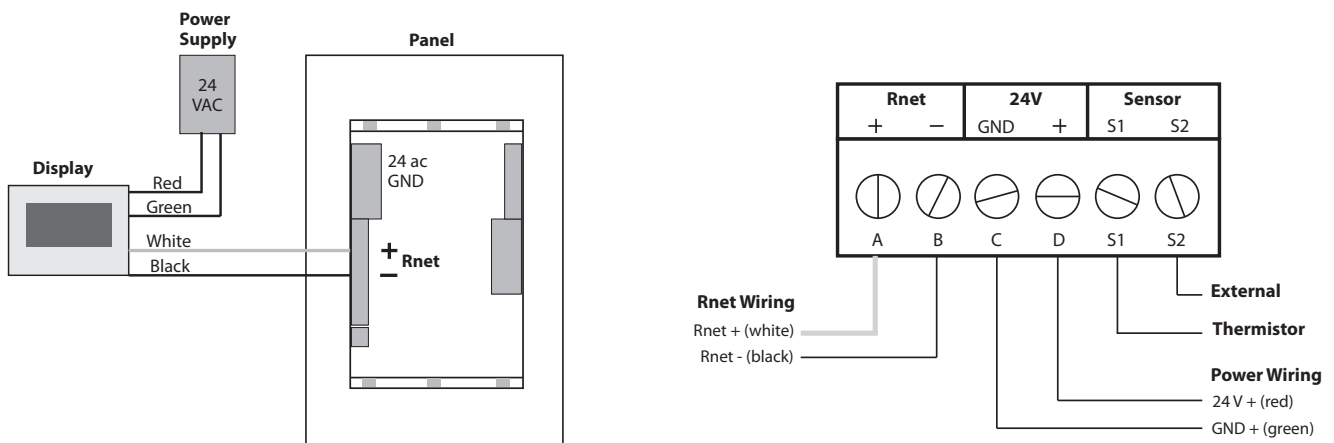
Figure 15: Equipment Touch wiring diagrams
