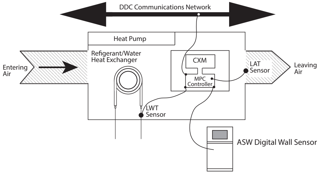
Figure 2: Typical System
