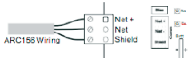
Figure 5: Wiring the ARC156
