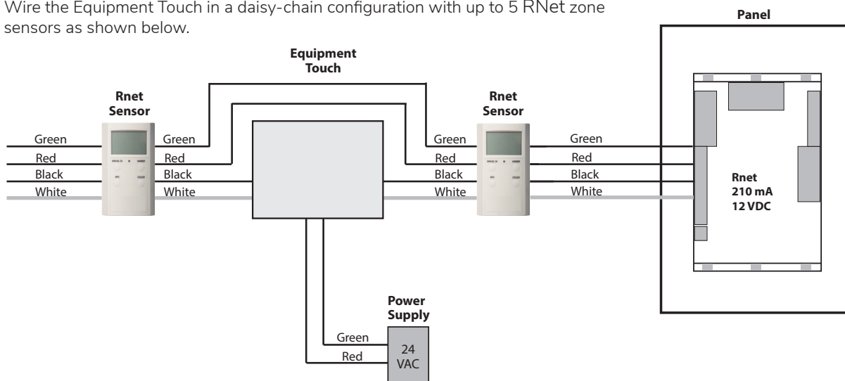
Figure 15: Equipment Touch wiring diagrams
