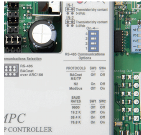
Figure 6: Communications Selections
